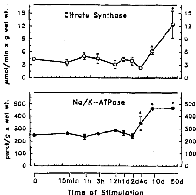
Fig. 1. Time-course of changes in citrate synthase activity and in the concentration of sarcolemmal Na + ,K + -ATPase as induced by chronic low-frequency stimulation in fast-twitch extensor digitorum longus muscle of rabbit. Values are means \pm S.E.M. n = 48 for zero time and 3–4 animals for each time point of stimulation. Asterisks mark significant ( P < 0.05 ) difference from zero time control.
